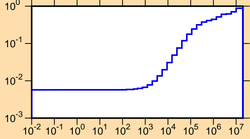
\mu vs. E for ^{123}\text{Sn}(\text{mt251})
