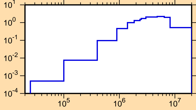
\sigma vs. E for ^{123}\text{Sn}(n,\text{inel.})
