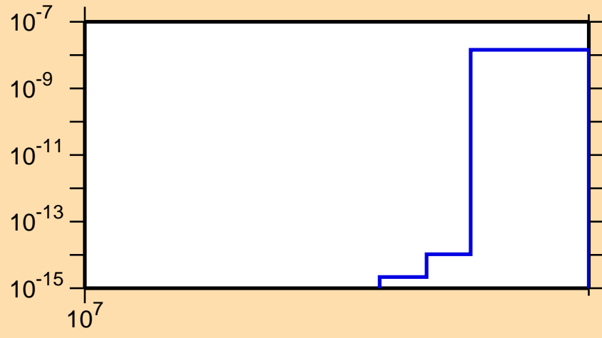
\sigma vs. E for ^{123}\text{Sn}(n,\text{nd})
