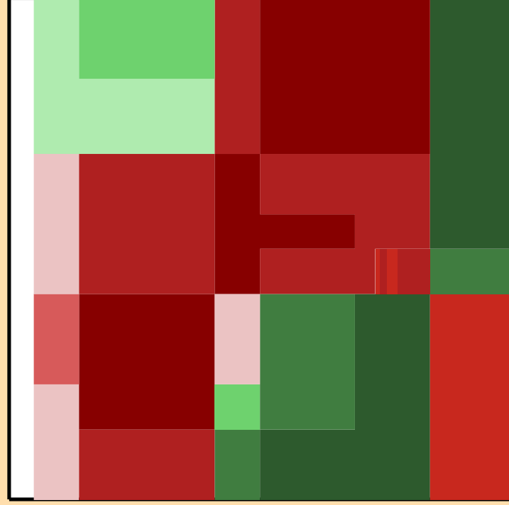
\Delta\sigma/\sigma vs. E for ^{123}\text{Sn}(n,2n)
