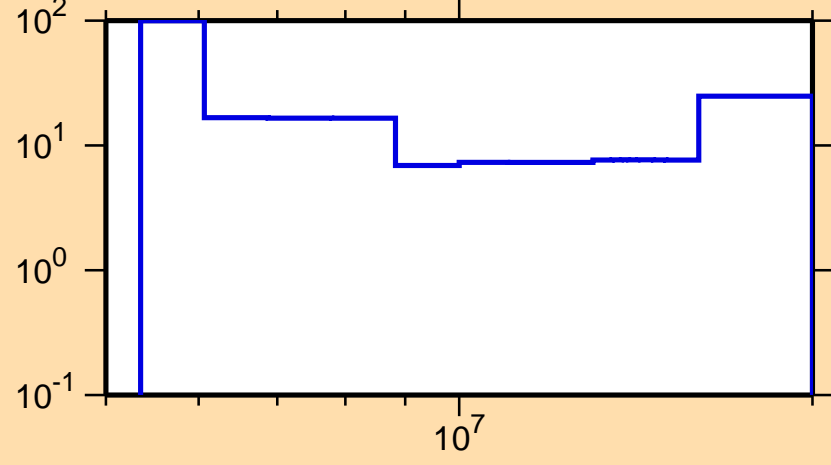
\Delta\sigma/\sigma vs. E for ^{123}\text{Sn}(n,2n)
