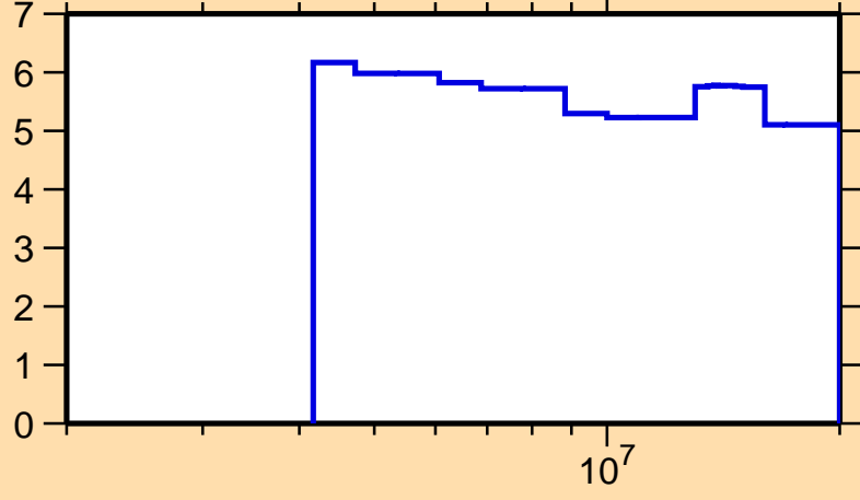
\Delta\sigma/\sigma vs. E for ^{123}\text{Sn}(n,\text{nonel.})
