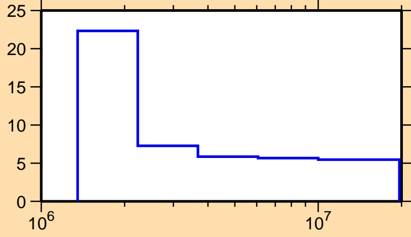
\Delta\sigma/\sigma vs. E for ^{123}\text{Sn}(n,\text{nonel.})
