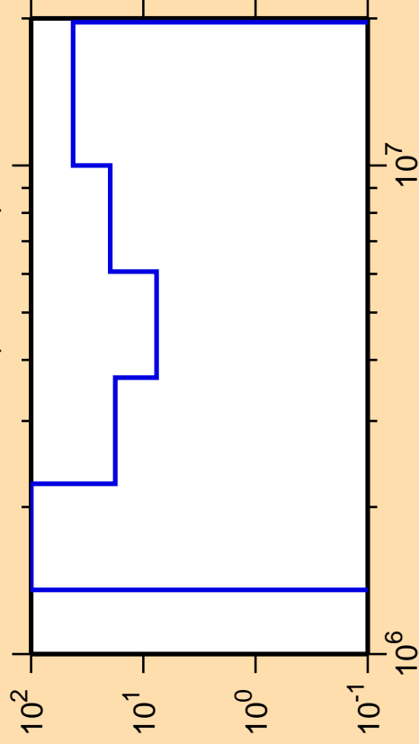
\Delta\sigma/\sigma vs. E for ^{123}\text{Sn}(n,n\text{cont.})
