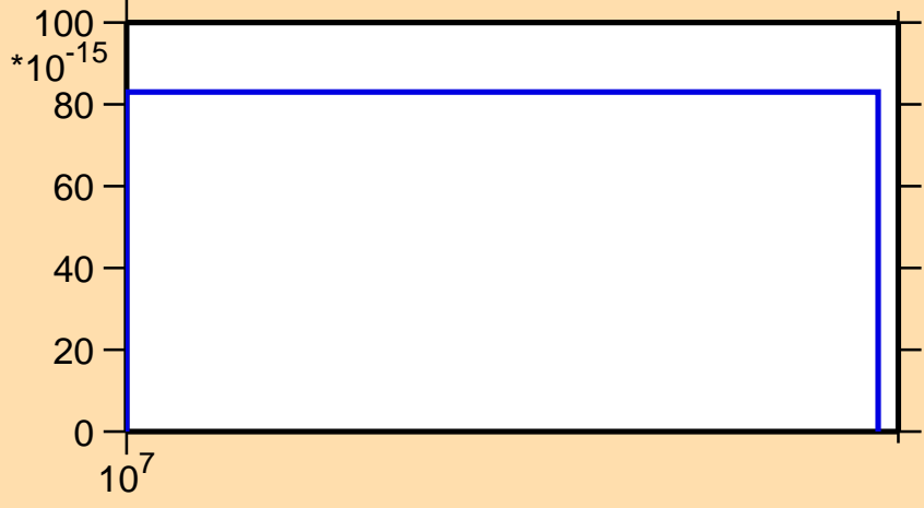
\sigma vs. E for ^{123}\text{Sn}(n,2n\alpha)
