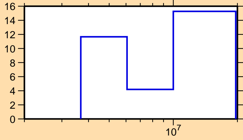
\Delta\sigma/\sigma vs. E for ^{123}\text{Sn}(n,el.)
