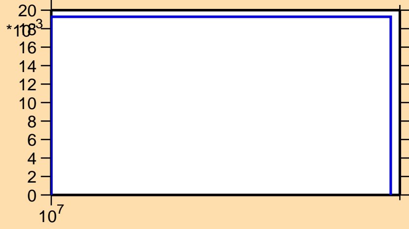
\sigma vs. E for ^{123}\text{Sn}(n,3n)
