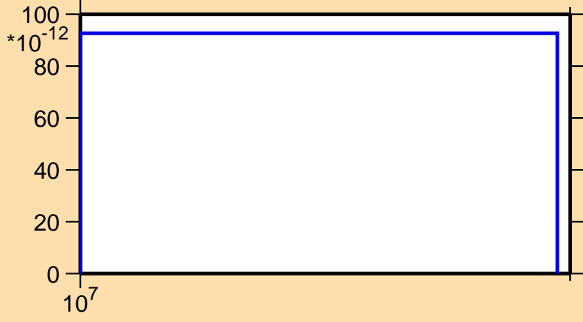
\sigma vs. E for ^{123}\text{Sn}(n,\text{nd})
