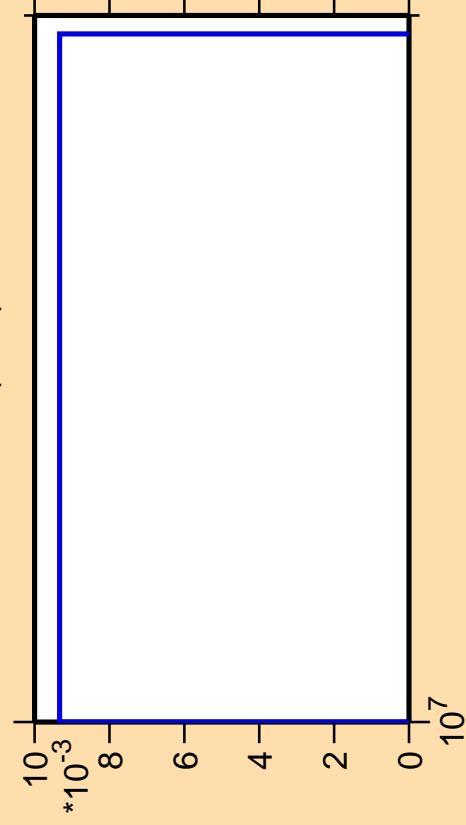
\Delta\sigma/\sigma vs. E for ^{123}\text{Sn}(n,nt)
