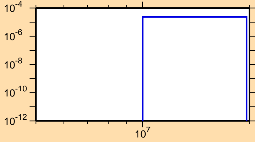
\sigma vs. E for ^{123}\text{Sn}(n,d)
