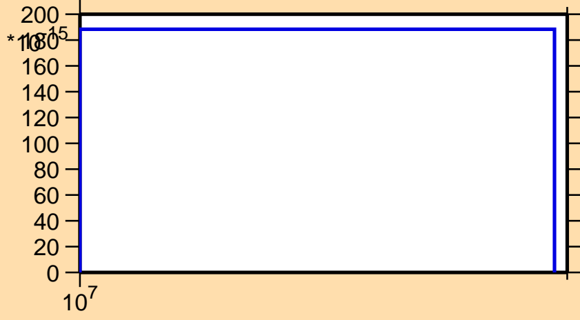
\sigma vs. E for ^{123}\text{Sn}(n,2np)
