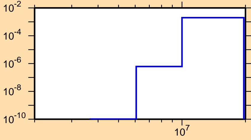
\sigma vs. E for ^{123}\text{Sn}(n,p)
