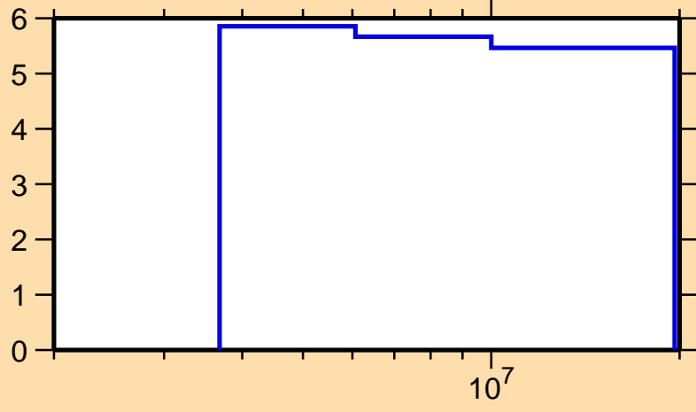
\Delta\sigma/\sigma vs. E for ^{123}\text{Sn}(n,\text{nonel.})
