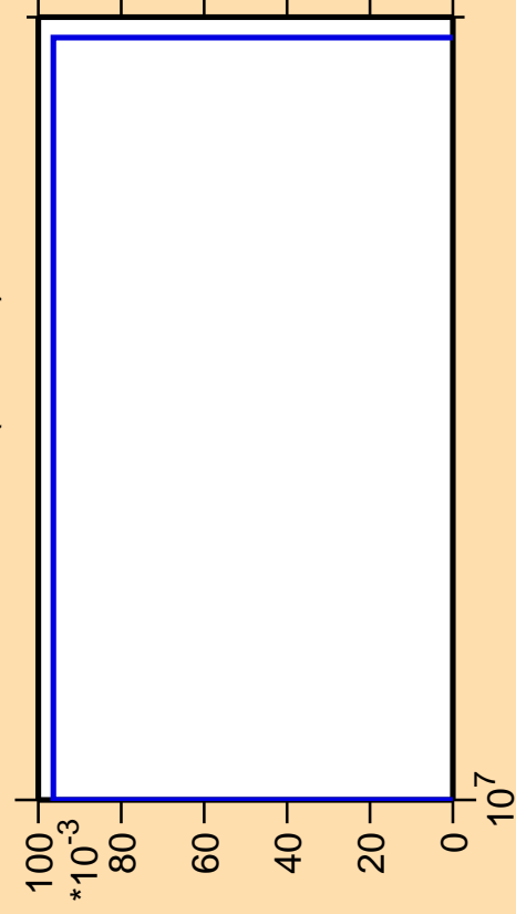
\Delta\sigma/\sigma vs. E for ^{123}\text{Sn}(n,2n\alpha)
