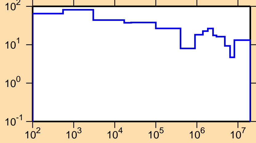
\Delta\sigma/\sigma vs. E for ^{123}\text{Sn}(n,\text{el.})
