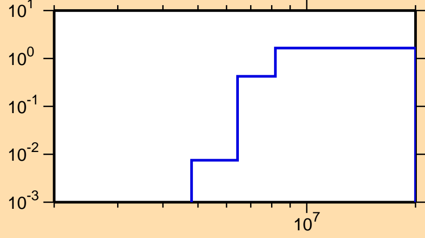
\sigma vs. E for ^{123}\text{Sn}(n,2n)
