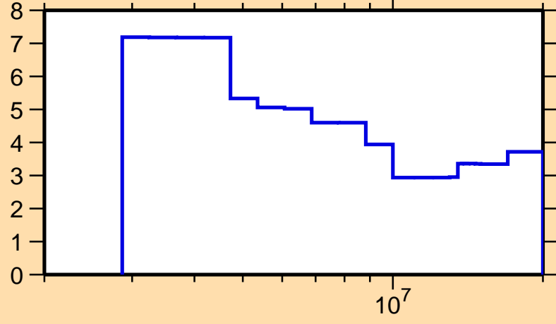
\Delta\sigma/\sigma vs. E for ^{124}\text{Sn}(n,\text{nonel.})
