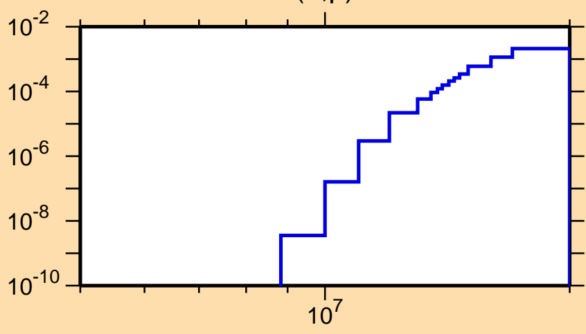
\sigma vs. E for ^{124}\text{Sn}(n,p)
