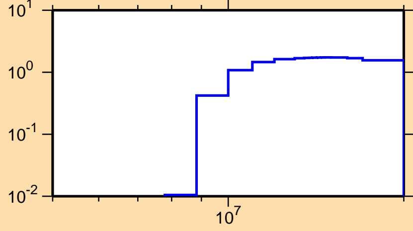
\sigma vs. E for ^{124}\text{Sn}(n,2n)
