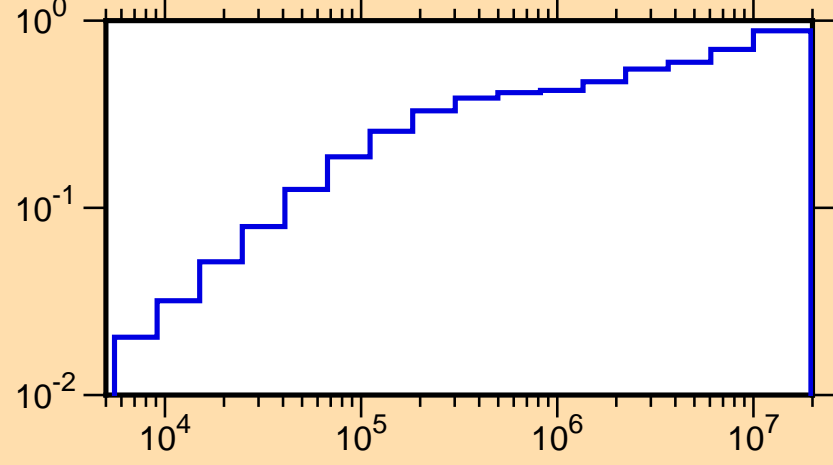
\mu vs. E for ^{124}\text{Sn}(\text{mt251})
