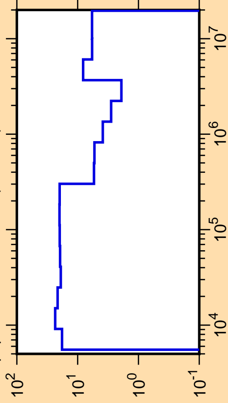
\Delta\mu/\mu vs. E for ^{124}\text{Sn}(\text{mt251})
