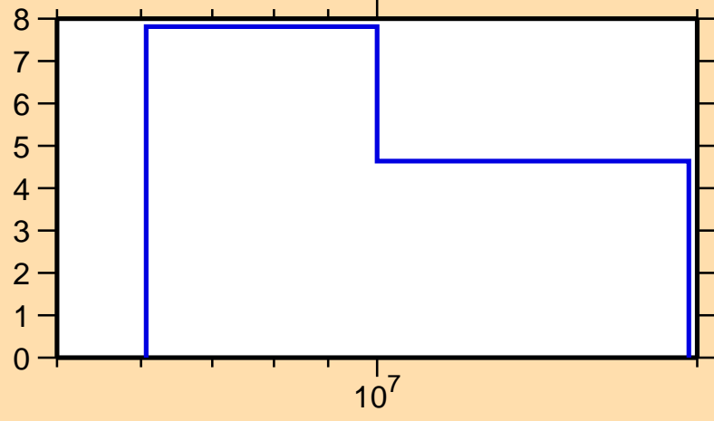
\Delta\sigma/\sigma vs. E for ^{124}\text{Sn}(n,el.)
