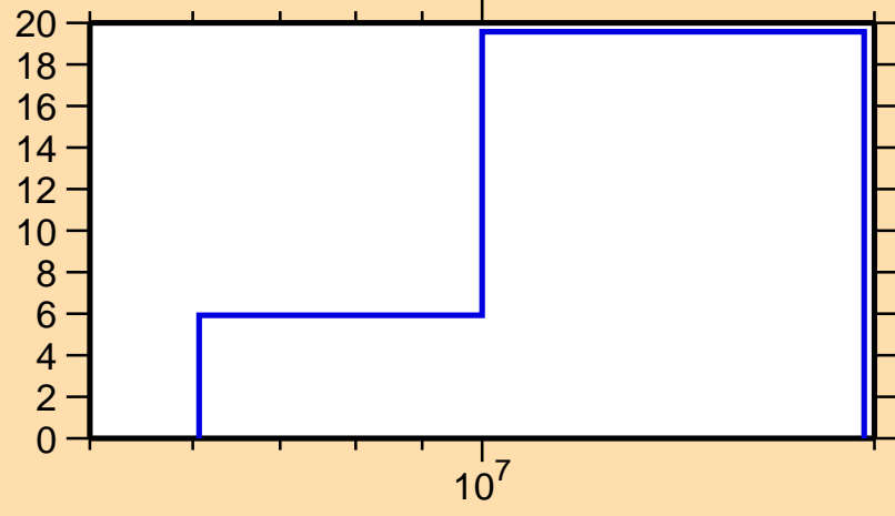
\Delta\sigma/\sigma vs. E for ^{124}\text{Sn}(n,ncont.)
