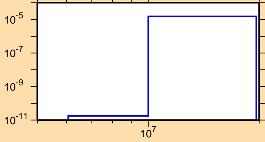
\sigma vs. E for ^{124}\text{Sn}(n,\alpha)
