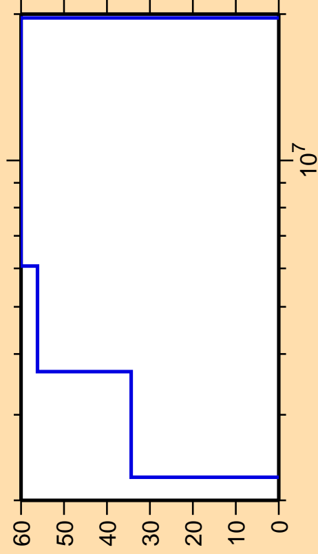
\Delta\sigma/\sigma vs. E for ^{124}\text{Sn}(n,\gamma)
