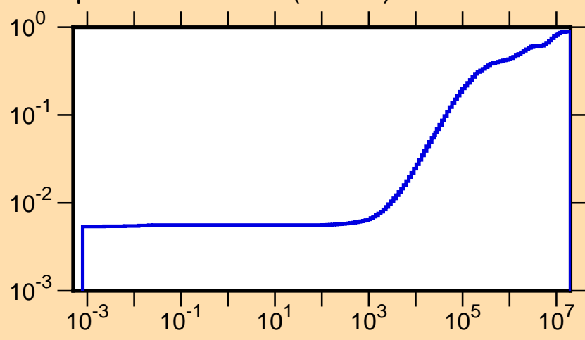
\mu vs. E for ^{125}\text{Sn}(\text{mt251})
