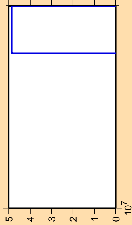
\Delta\sigma/\sigma vs. E for ^{125}\text{Sn}(n,2np)
