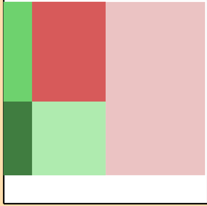
\Delta\sigma/\sigma vs. E for ^{125}\text{Sn}(n,\gamma)
