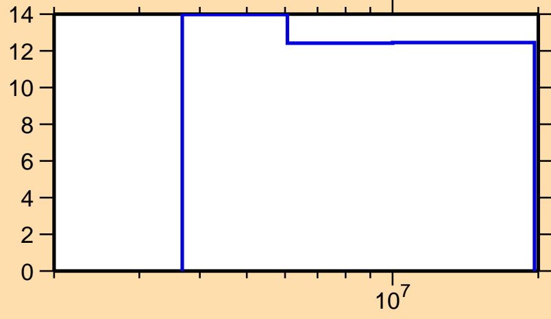
\Delta\sigma/\sigma vs. E for ^{125}\text{Sn}(n,el.)
