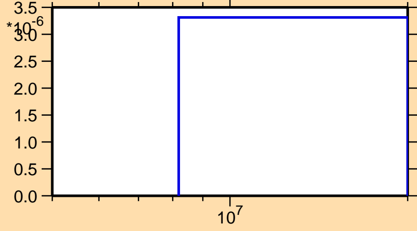
\sigma vs. E for ^{125}\text{Sn}(n,d)
