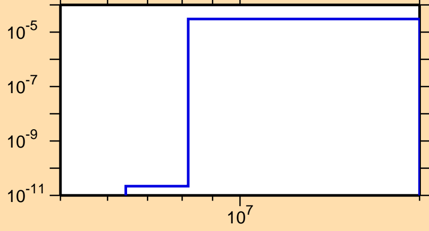
\sigma vs. E for ^{125}\text{Sn}(n,\alpha)
