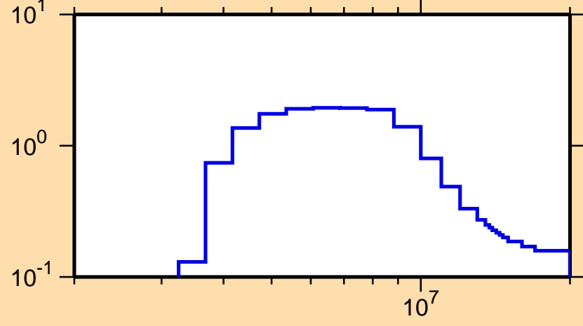
\sigma vs. E for ^{126}\text{Sn}(n,n_{\text{cont}}) .
