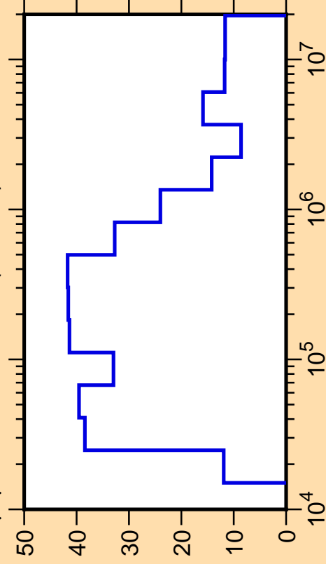
\Delta\mu/\mu vs. E for ^{126}\text{Sn}(\text{mt251})
