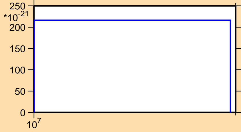
\sigma vs. E for ^{126}\text{Sn}(n,nd)
