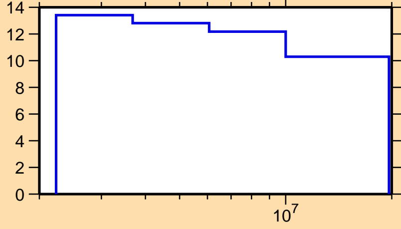
\Delta\sigma/\sigma vs. E for ^{126}\text{Sn}(n,n\text{inel.})
