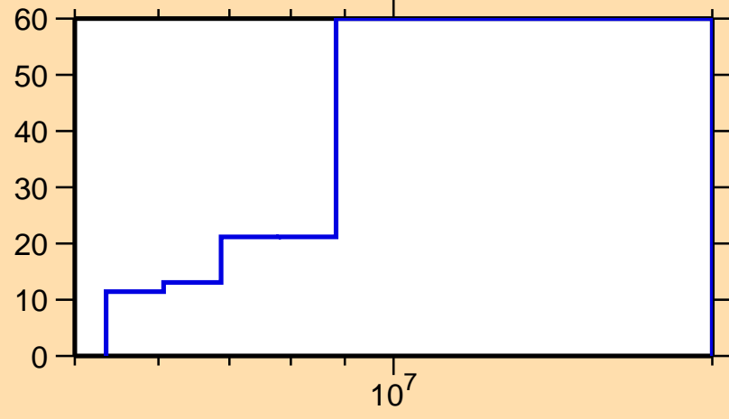
\Delta\sigma/\sigma vs. E for ^{127}\text{Sn}(n,ncont.)
