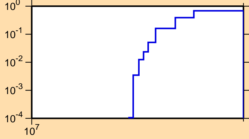
\sigma vs. E for ^{127}\text{Sn}(n,3n)
