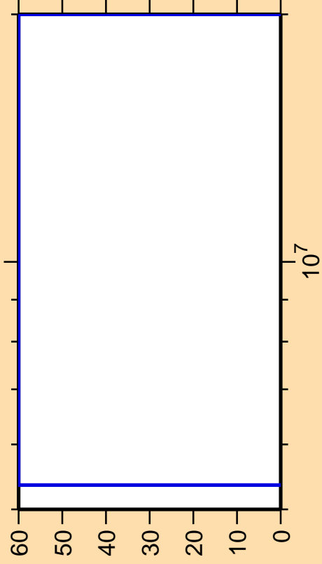
\Delta\sigma/\sigma vs. E for ^{127}\text{Sn}(n,n_1)
