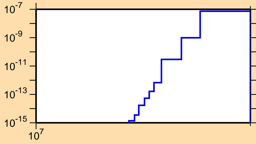
\sigma vs. E for ^{127}\text{Sn}(n,n\alpha)
