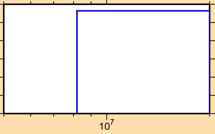
\sigma vs. E for ^{127}\text{Sn}(n,np)
