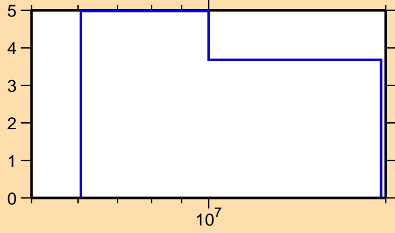
\Delta\sigma/\sigma vs. E for ^{127}\text{Sn}(n,el.)
