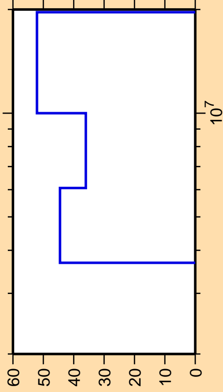
\Delta\sigma/\sigma vs. E for ^{128}\text{Sn}(n,n\text{cont.})
