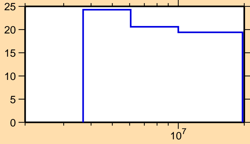
\Delta\sigma/\sigma vs. E for ^{128}\text{Sn}(n,n\text{onel.})
