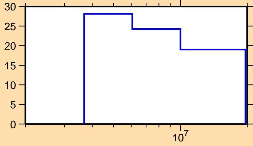
\Delta\sigma/\sigma vs. E for ^{128}\text{Sn}(n,el.)
