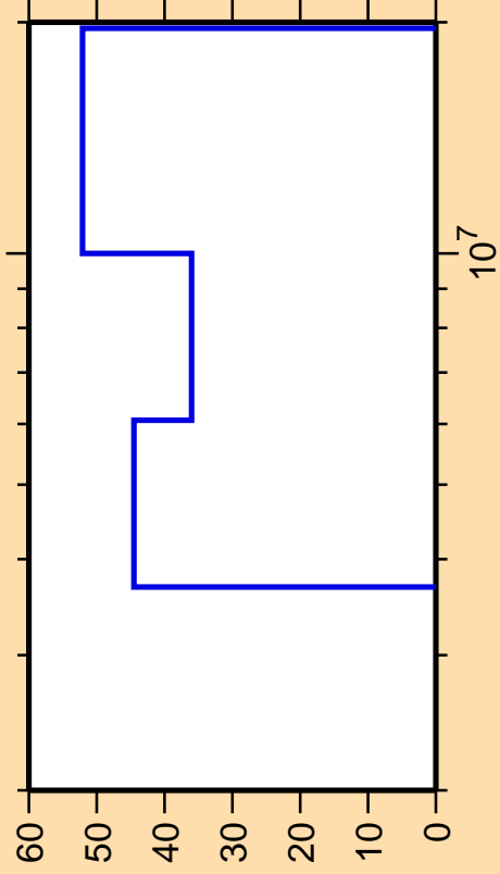
\Delta\sigma/\sigma vs. E for ^{128}\text{Sn}(n,ncont.)
