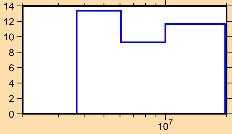
\Delta\sigma/\sigma vs. E for ^{128}\text{Sn}(n,tot.)
