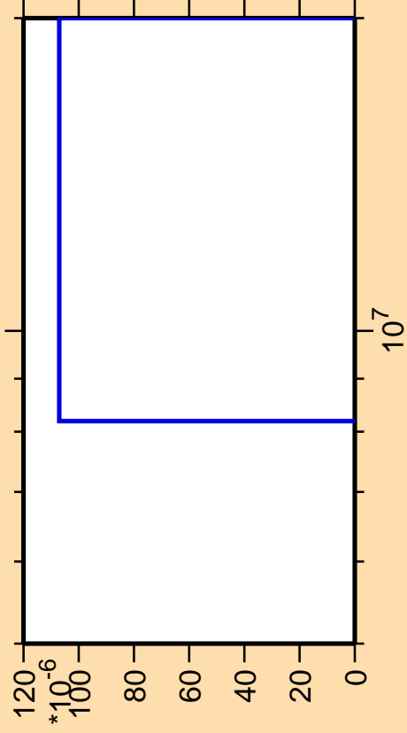
\Delta\sigma/\sigma vs. E for ^{128}\text{Sn}(n,\text{nd})
