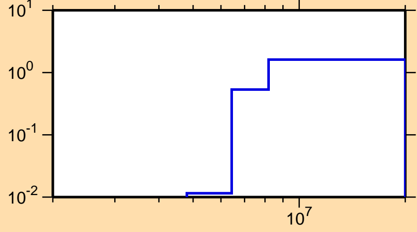
\sigma vs. E for ^{128}\text{Sn}(n,2n)
