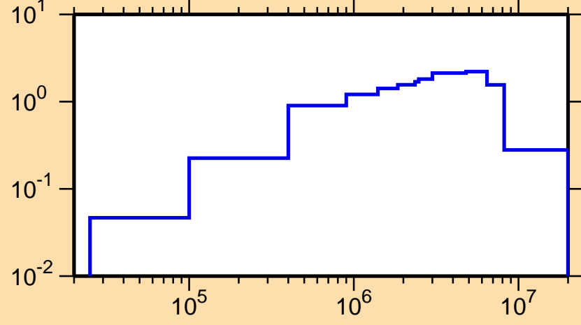
\sigma vs. E for ^{128}\text{Sn}(n,\text{inel.})
