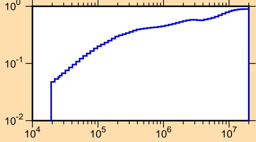
\mu vs. E for ^{129}\text{Sn}(\text{mt251})
