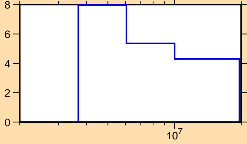
\Delta\sigma/\sigma vs. E for ^{129}\text{Sn}(n,\text{nonel.})
