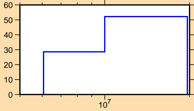
\Delta\sigma/\sigma vs. E for ^{129}\text{Sn}(n,ncont.)
