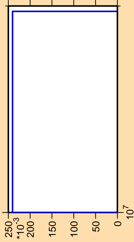
\Delta\sigma/\sigma vs. E for ^{129}\text{Sn}(n,nd)
