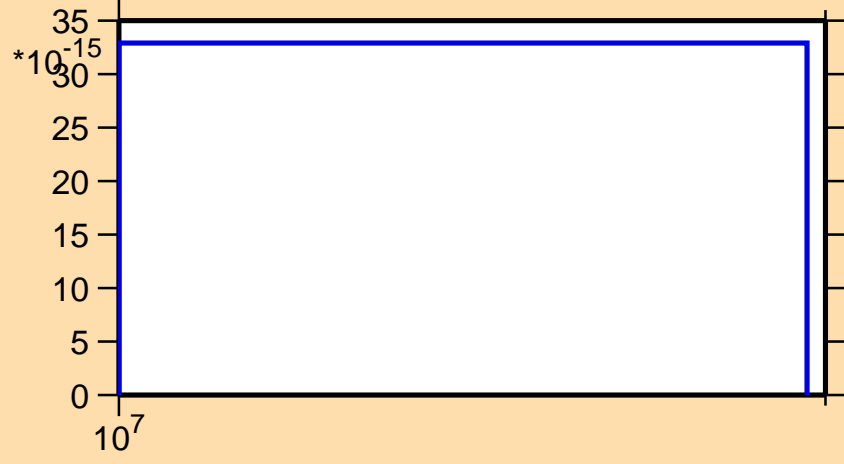
\sigma vs. E for ^{129}\text{Sn}(n,nd)
