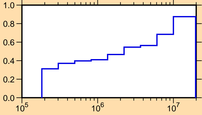
\mu vs. E for ^{130}\text{Sn}(\text{mt251})
