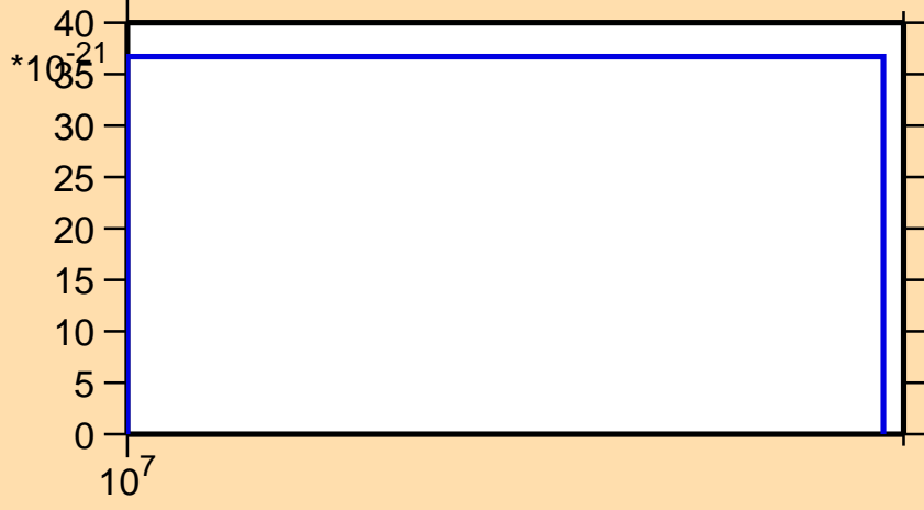
\sigma vs. E for ^{130}\text{Sn}(n,\text{nd})
