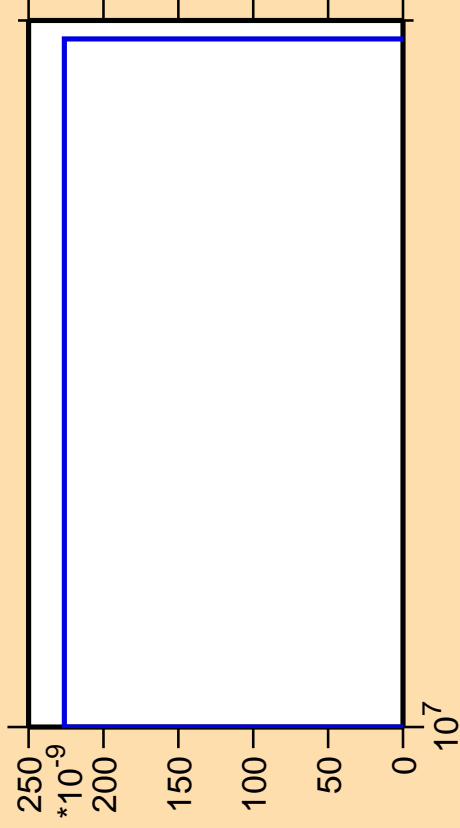
\Delta\sigma/\sigma vs. E for ^{130}\text{Sn}(n,\text{nd})
