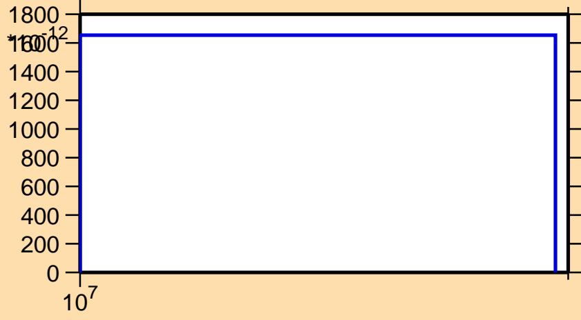
\sigma vs. E for ^{130}\text{Sn}(n,t)
