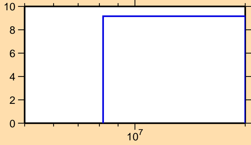
\Delta\sigma/\sigma vs. E for ^{130}\text{Sn}(n,el.)
