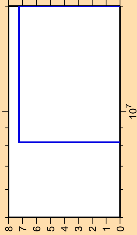
\Delta\sigma/\sigma vs. E for ^{130}\text{Sn}(n,n\alpha)
