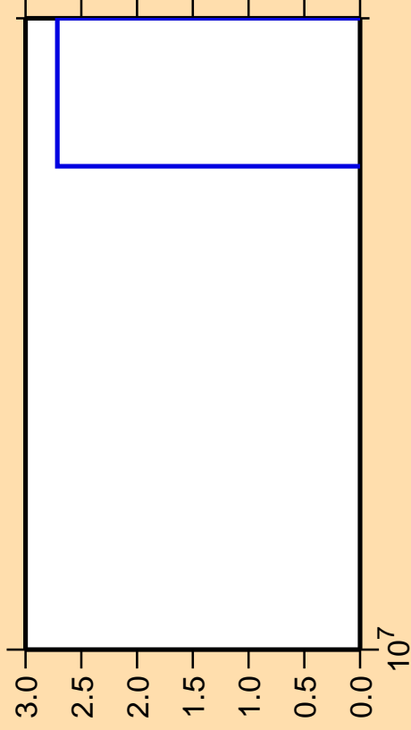
\Delta\sigma/\sigma vs. E for ^{130}\text{Sn}(n,nd)
