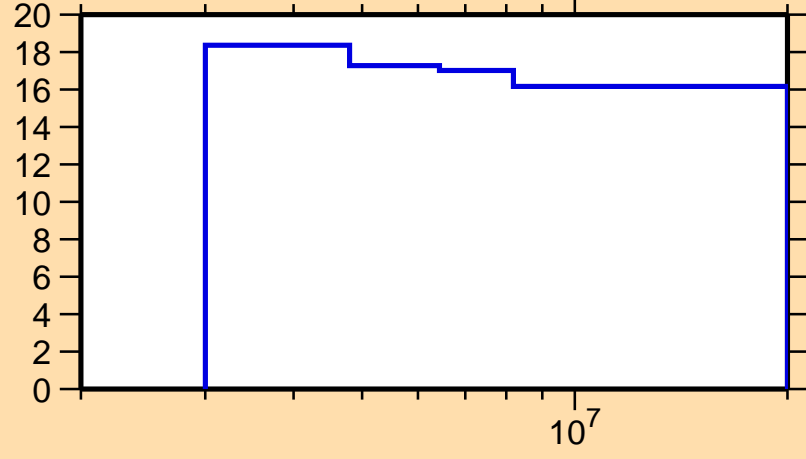
\Delta\sigma/\sigma vs. E for ^{130}\text{Sn}(n,n\text{nonel.})
