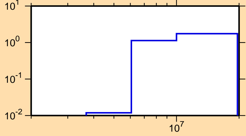
\sigma vs. E for ^{131}\text{Sn}(n,2n)
