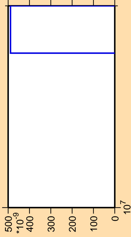
\Delta\sigma/\sigma vs. E for ^{131}\text{Sn}(n,2np)
