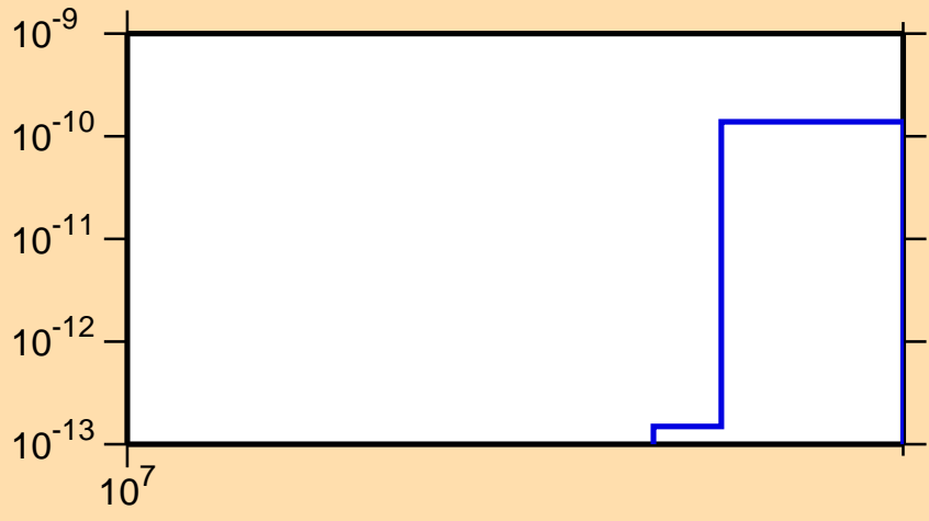
\sigma vs. E for ^{131}\text{Sn}(n,n\alpha)
