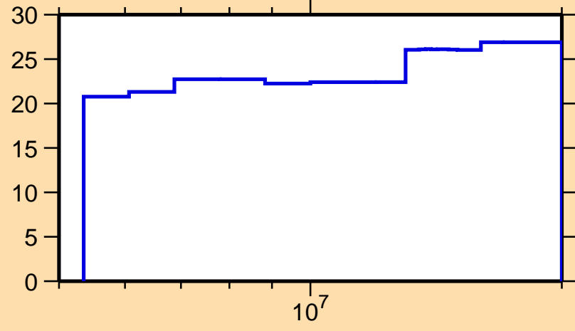
\Delta\sigma/\sigma vs. E for ^{131}\text{Sn}(n,n\text{onel.})
