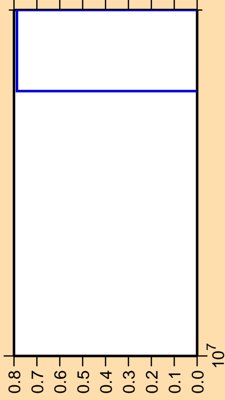
\Delta\sigma/\sigma vs. E for ^{131}\text{Sn}(n,nd)
