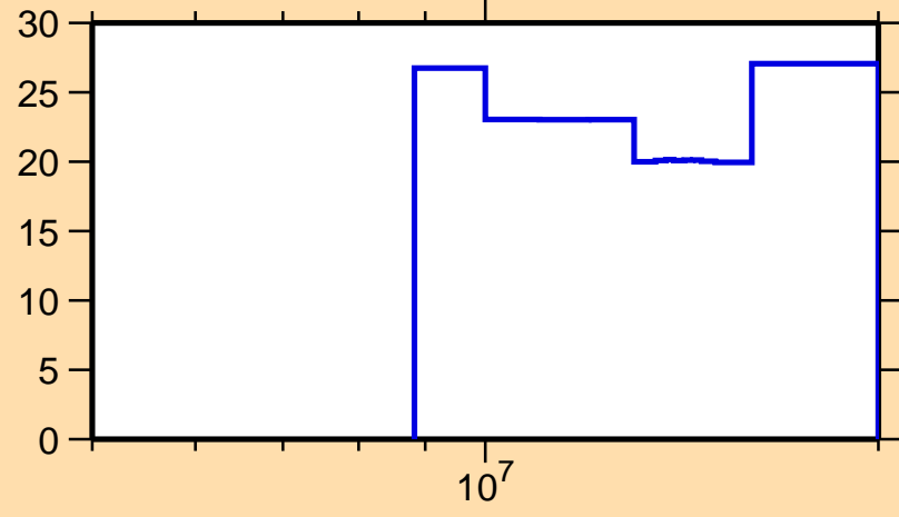
\Delta\sigma/\sigma vs. E for ^{131}\text{Sn}(n,el.)
