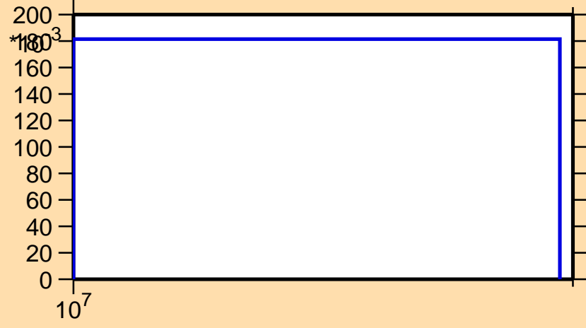
\sigma vs. E for ^{131}\text{Sn}(n,3n)
