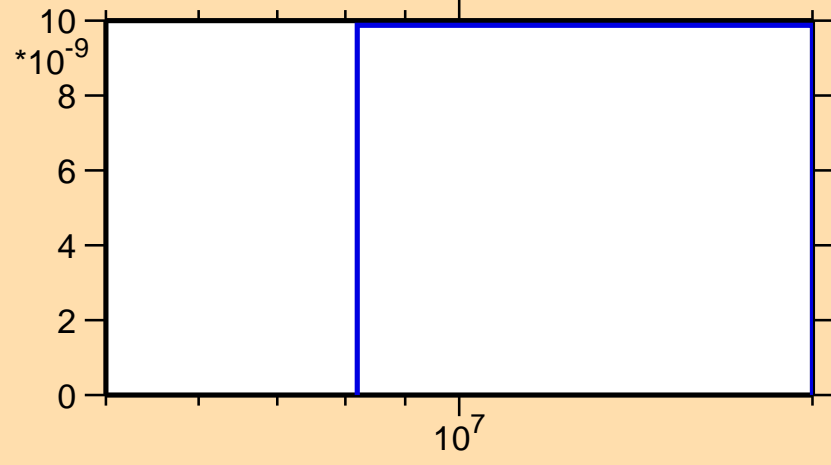
\sigma vs. E for ^{131}\text{Sn}(n,\alpha)
