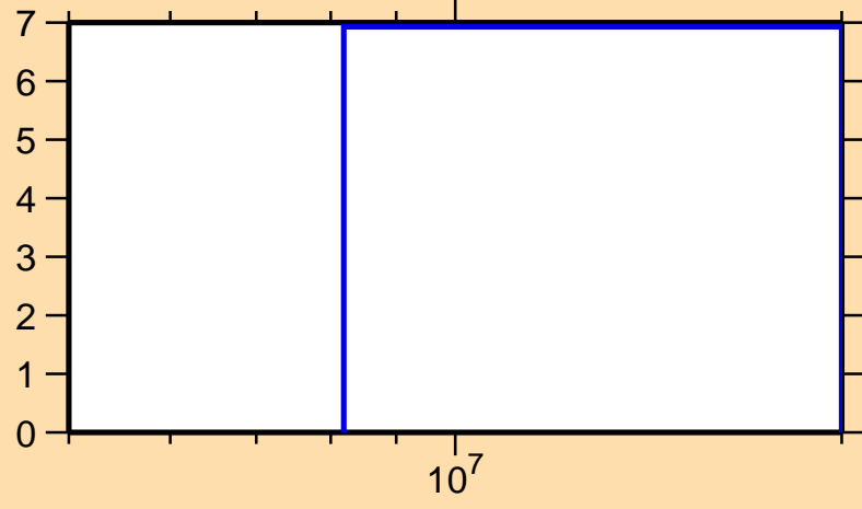
\Delta\sigma/\sigma vs. E for ^{131}\text{Sn}(n,\text{tot.})
