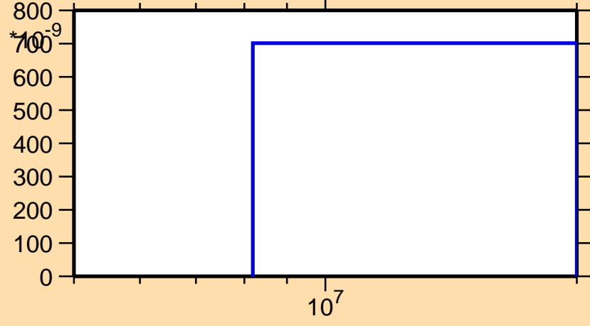
\sigma vs. E for ^{131}\text{Sn}(n,p)
