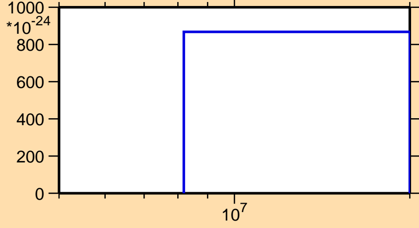
\sigma vs. E for ^{131}\text{Sn}(n,2np)
