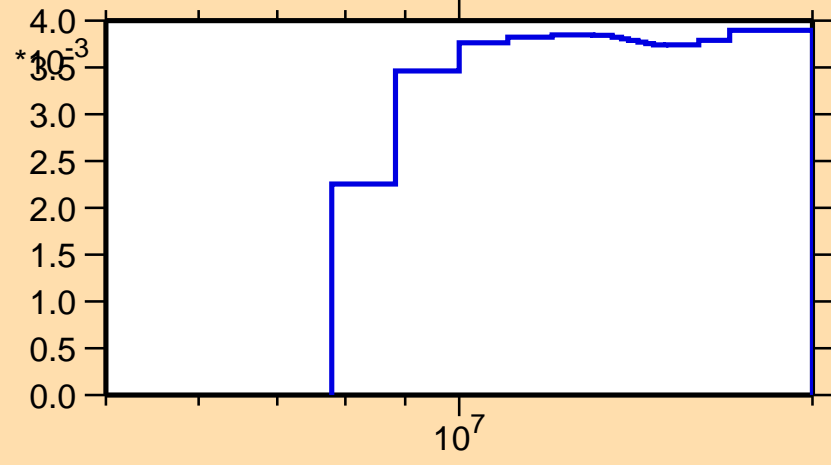
\sigma vs. E for ^{132}\text{Sn}(n,n\text{cont.})
