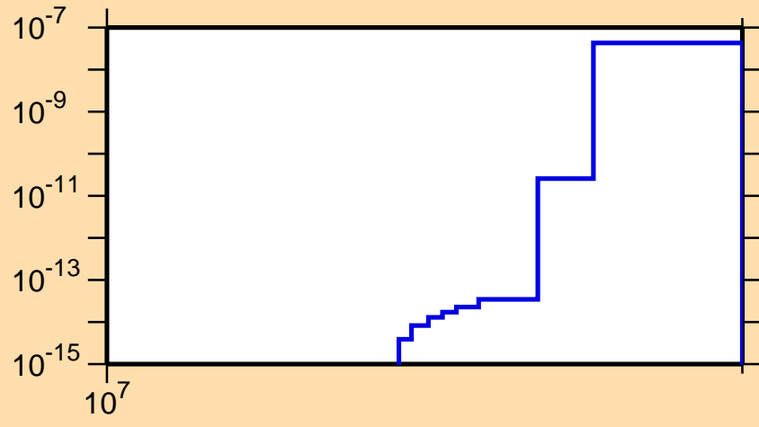
\sigma vs. E for ^{132}\text{Sn}(n,t)
