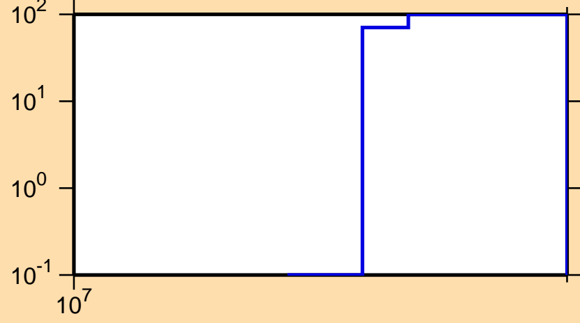
\Delta\sigma/\sigma vs. E for ^{132}\text{Sn}(n,p)
