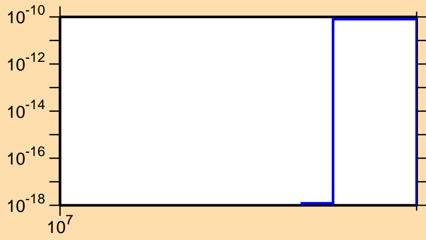
\sigma vs. E for ^{132}\text{Sn}(n,np)
