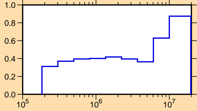
\mu vs. E for ^{132}\text{Sn}(\text{mt251})
