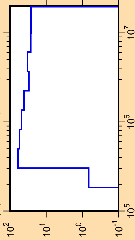
\Delta\mu/\mu vs. E for ^{132}\text{Sn}(\text{mt251})
