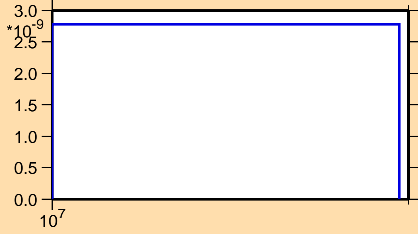
\sigma vs. E for ^{132}\text{Sn}(n,d)
