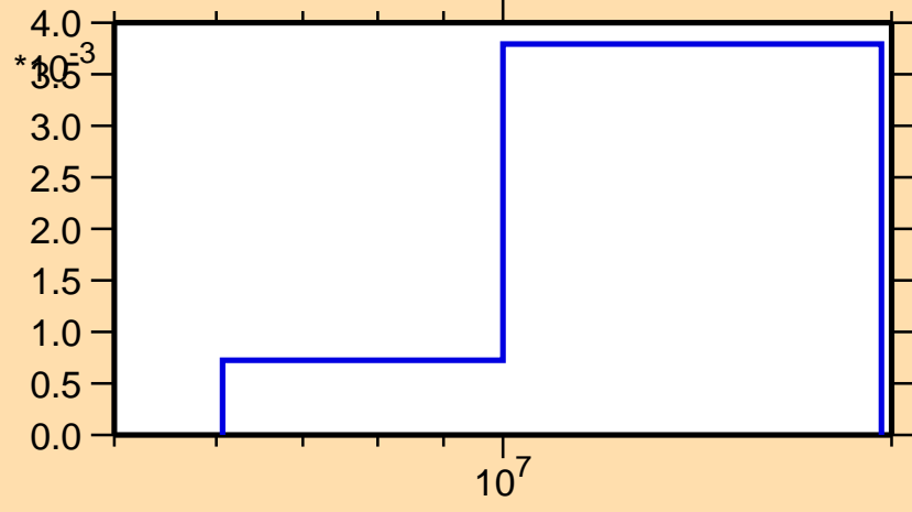
\sigma vs. E for ^{132}\text{Sn}(n,n\text{cont.})
