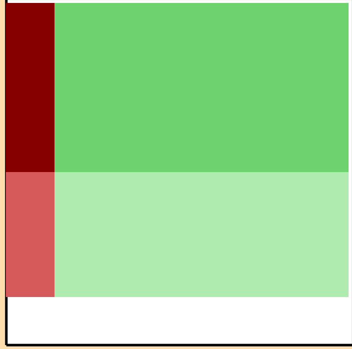
\Delta\sigma/\sigma vs. E for ^{132}\text{Sn}(n,n_1)
