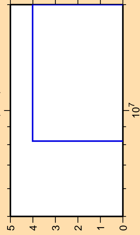
\Delta\sigma/\sigma vs. E for ^{133}\text{Sn}(n,nt)
