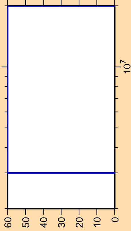
\Delta\sigma/\sigma vs. E for ^{133}\text{Sn}(n,n_{\text{cont}}) .
