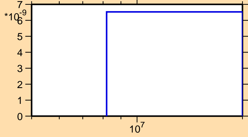
\sigma vs. E for ^{133}\text{Sn}(n,\alpha)
