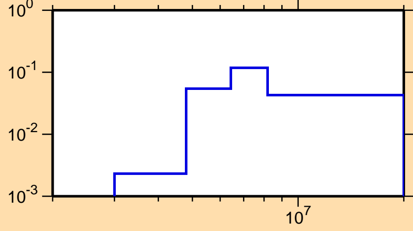
\sigma vs. E for ^{133}\text{Sn}(n,n\text{cont.})
