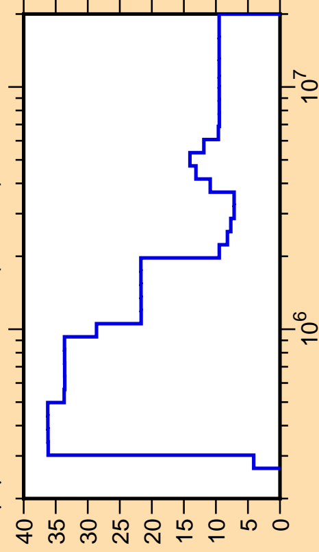
\Delta\mu/\mu vs. E for ^{134}\text{Sn}(\text{mt251})
