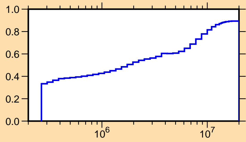
\mu vs. E for ^{134}\text{Sn}(\text{mt251})
