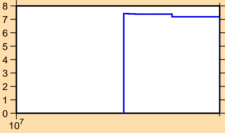
\Delta\sigma/\sigma vs. E for ^{134}\text{Sn}(n,\text{nonel.})
