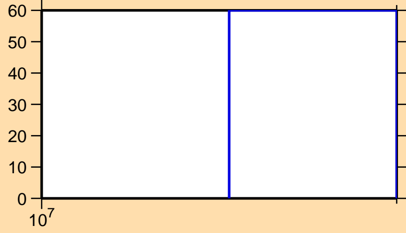
\Delta\sigma/\sigma vs. E for ^{134}\text{Sn}(n,ncont.)
