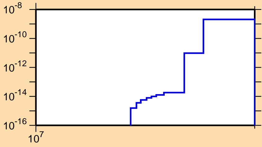
\sigma vs. E for ^{134}\text{Sn}(n,nt)
