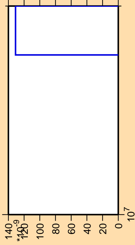
\Delta\sigma/\sigma vs. E for ^{134}\text{Sn}(\text{mt } 11)
