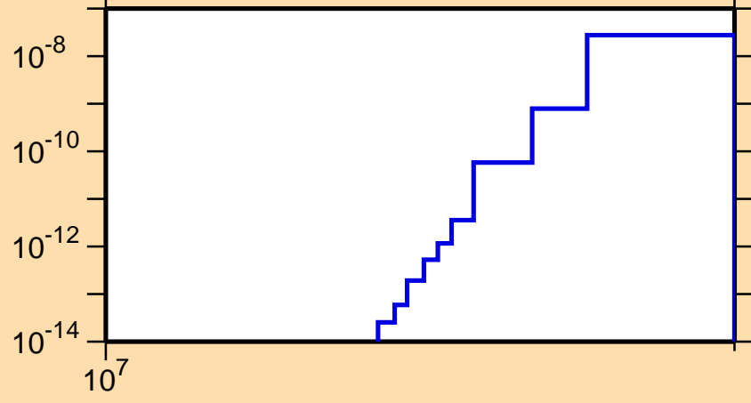
\sigma vs. E for ^{134}\text{Sn}(n,n\alpha)
