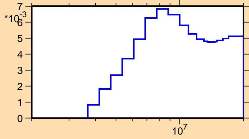
\sigma vs. E for ^{134}\text{Sn}(n,n\text{cont.})
