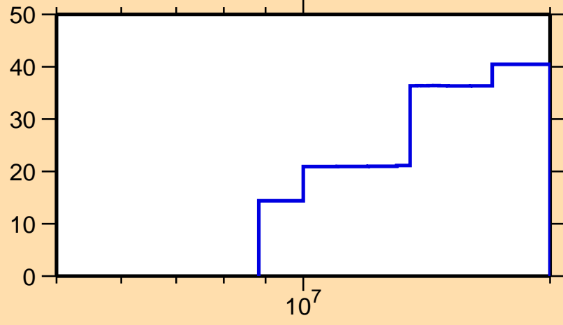
\Delta\sigma/\sigma vs. E for ^{134}\text{Sn}(n,2n)
