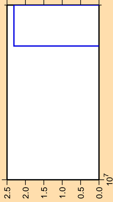
\Delta\sigma/\sigma vs. E for ^{134}\text{Sn}(n,nd)
