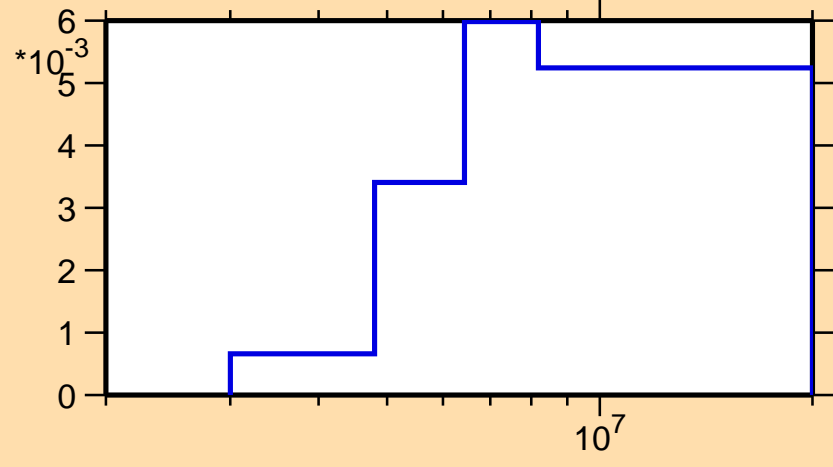
\sigma vs. E for ^{134}\text{Sn}(n,n\text{cont.})
