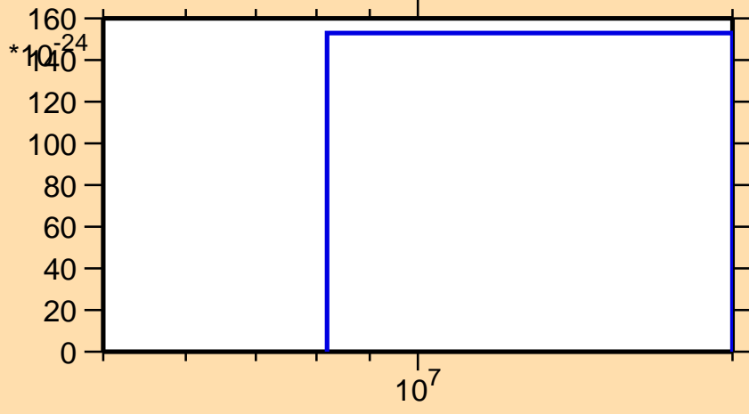
\sigma vs. E for ^{134}\text{Sn}(\text{mt } 11)
