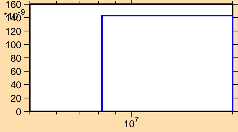
\sigma vs. E for ^{134}\text{Sn}(n,t)
