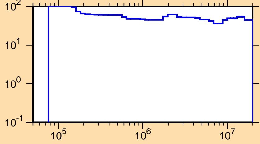
\Delta\sigma/\sigma vs. E for ^{81}\text{Sr}(n,\text{inel.})
