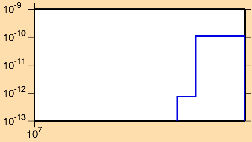
\sigma vs. E for ^{81}\text{Sr}(\text{mt117})
