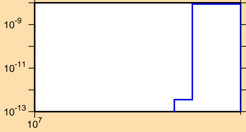
\sigma vs. E for ^{81}\text{Sr}(n,2n\alpha)
