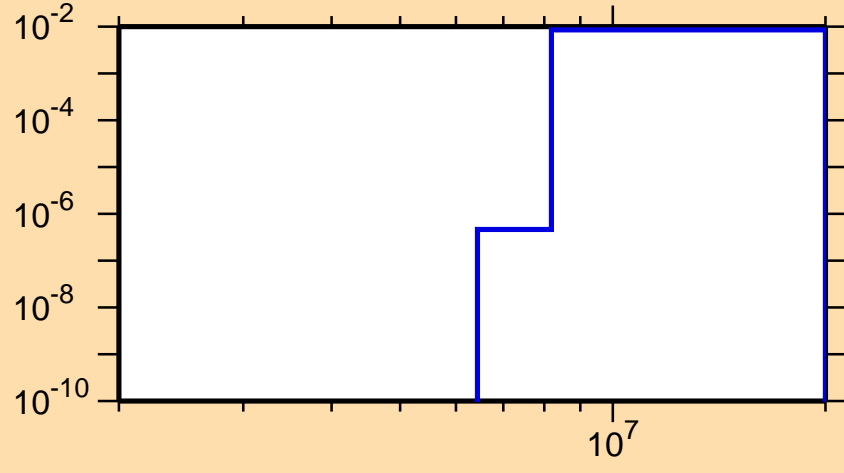
\sigma vs. E for ^{81}\text{Sr}(n,d)
