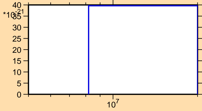
\sigma vs. E for ^{81}\text{Sr}(n,nt)
