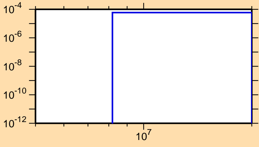
\sigma vs. E for ^{81}\text{Sr}(n,t)
