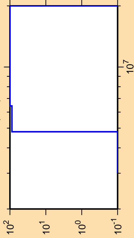
\Delta\sigma/\sigma vs. E for ^{81}\text{Sr}(n,d)
