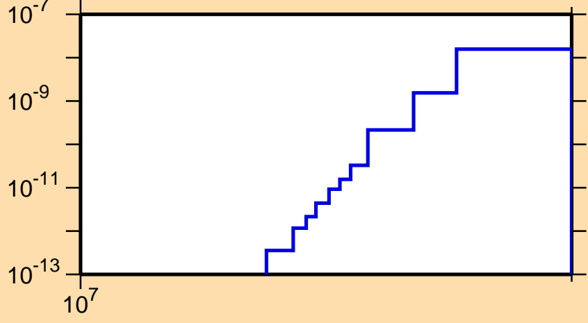
\sigma vs. E for ^{159}\text{Ta}(\text{mt } 34)
