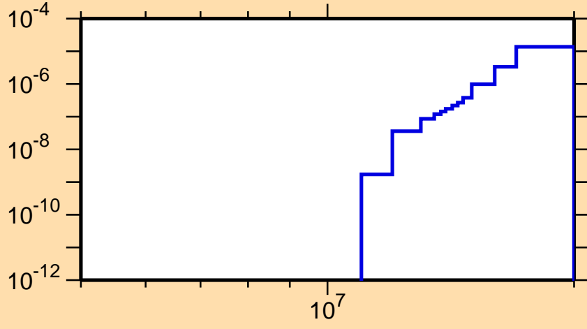
\sigma vs. E for ^{159}\text{Ta}(n,2n\alpha)
