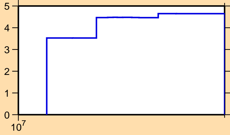
\Delta\sigma/\sigma vs. E for ^{159}\text{Ta}(n,\text{nonel.})
