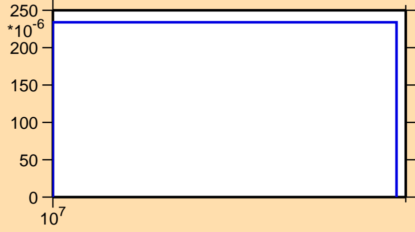
\sigma vs. E for ^{159}\text{Ta}(n,2np)
