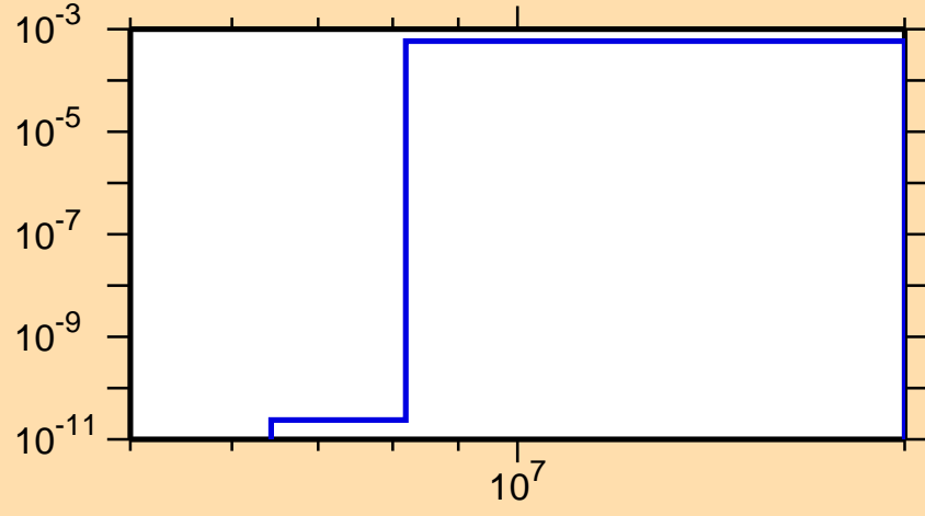
\sigma vs. E for ^{159}\text{Ta}(n,t)
