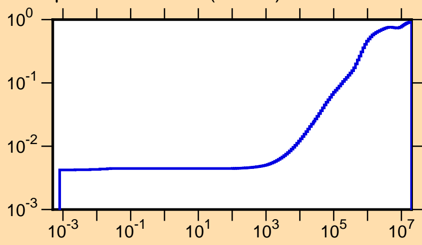
\mu vs. E for ^{160}\text{Ta}(\text{mt251})
