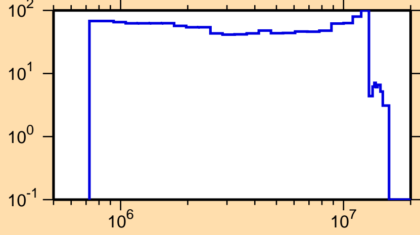
\Delta\sigma/\sigma vs. E for ^{160}\text{Ta}(n,n_1)
