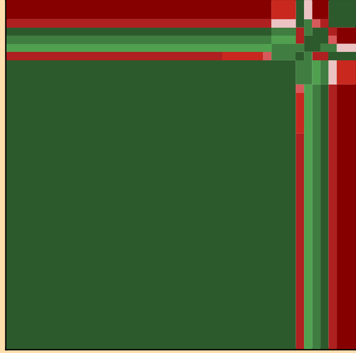
\mu vs. E for ^{160}\text{Ta}(\text{mt251})
