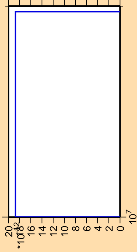
\Delta\sigma/\sigma vs. E for ^{160}\text{Ta} (mt 11)
