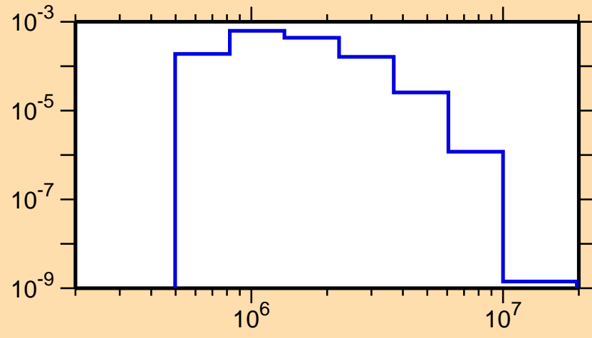
\sigma vs. E for ^{160}\text{Ta}(n,n_3)
