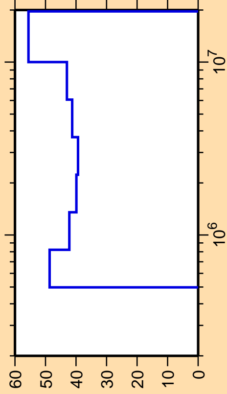
\Delta\sigma/\sigma vs. E for ^{160}\text{Ta}(n,n_3)
