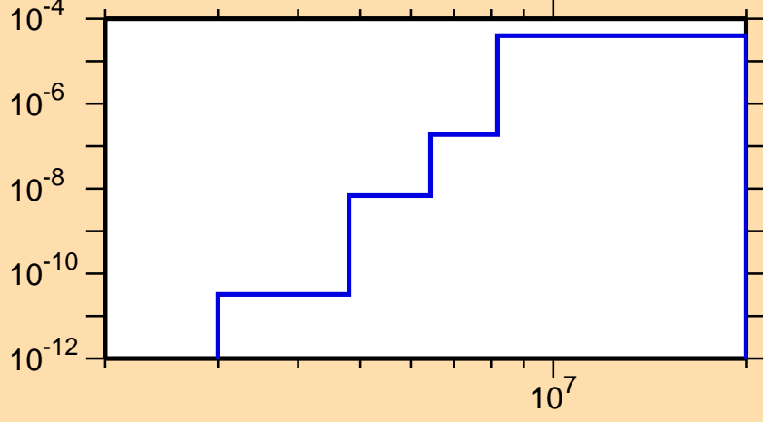
\sigma vs. E for ^{160}\text{Ta}(\text{mt117})
