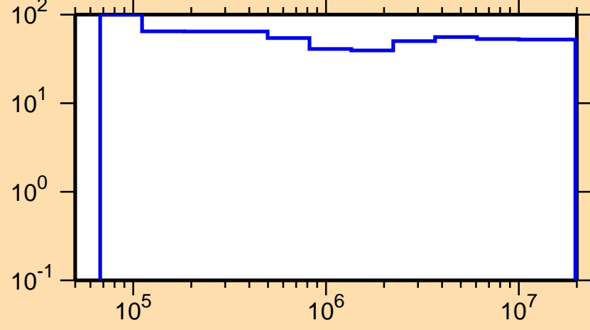
\Delta\sigma/\sigma vs. E for ^{161}\text{Ta}(n,n_1)
