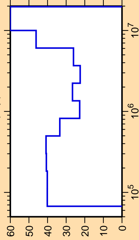
\Delta\sigma/\sigma vs. E for ^{161}\text{Ta}(n,p)
